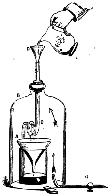
Fig. 170. A. Funnel and filter containing the sulphide of copper, &c. B. Gas jar fitted with a cork and glass tube in neck; the tube is bent round at C, so that the coal gas may not escape. D. The funnel by which the water is poured in to wash the sulphide of copper, and by turning the beaker round that supplies the funnel, every part of the filter may be washed. G. Gas-pipe connected with the coal-gas fittings. The arrows denote the entry of the gas.
